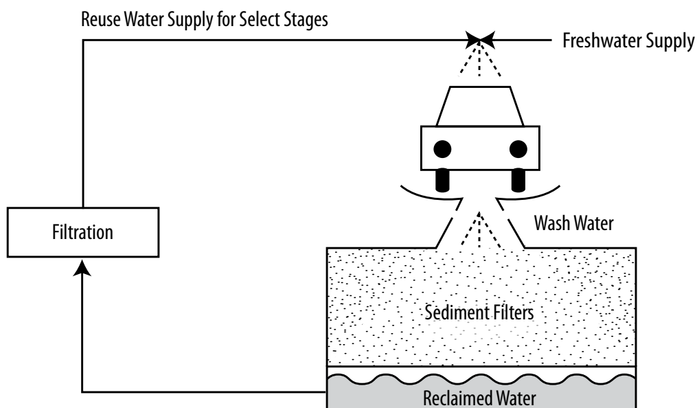
Figure 5-4. Vehicle Wash Water Reclamation System
