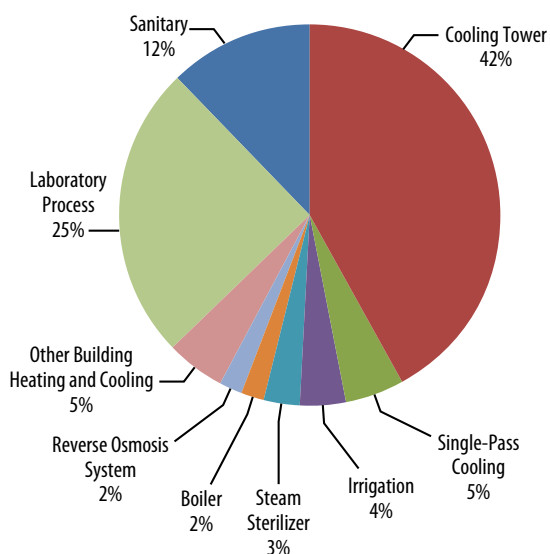
Figure 7-1. Laboratory Water Consumption
